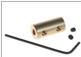
In-line Coupling. 8mm-8mm. Dia. 12.67mm x 24.8mm. 23g Part No: 919D1/8
