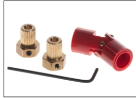
Universal Couplings. 12.5mm dia. 44mm length. Part No: 1105/60 6mm - 6mm. See Universal Couplings Page for full range of combinations
