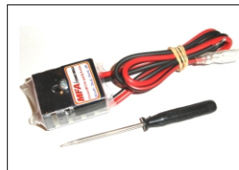
Voltage Regulator. (6-15v DC Input. 4v-12v output). 26mm x 31mm x 15.5mm. 30g Part No: 919D2
