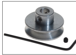
Pulley. 2mm I.D. (25mm dia. x 14.75mm) (Aluminium). 12g Part No: 918D2
