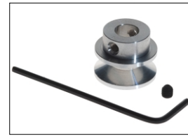
Pulley. 2mm I.D. (16mm dia. x 13.6mm) (Aluminium). 6g Part No: 918D3
